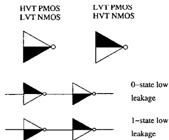
Figure 2: Staggered threshold voltage buffers.
