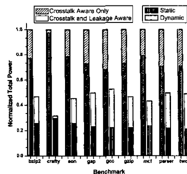
Figure 6: Power savings for the described crosstalk and leakage-aware encoding vs. crosstalk-only encoding [5].
