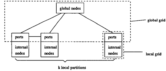
Figure 1: Hierarchical power network analysis
