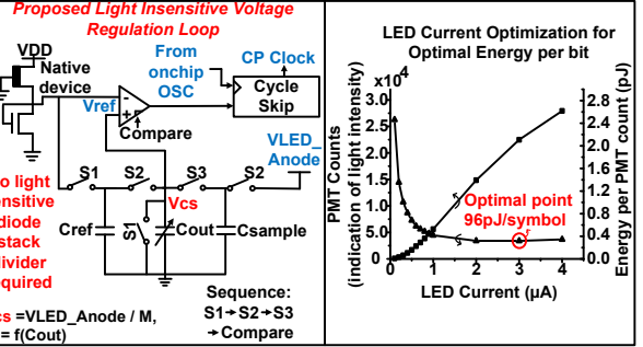
Figure 4. Circuit implementation of optical transmitter subsystem
