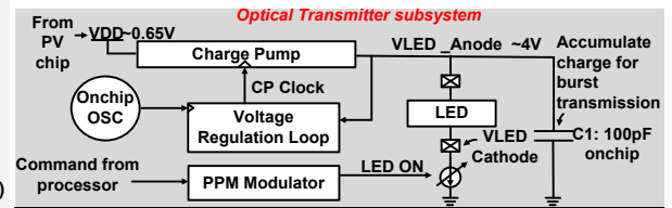
Figure 2. System architecture of CTS
