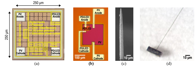
Fig. 9. Photos of StiMote components: (a) CMOS chip in 180 nm process, (b) GaAs PV-PD/LED cell, (c) PtIr-stacked CF electrode, and (d) a dummy mote with stacked CMOS and GaAs layers.
