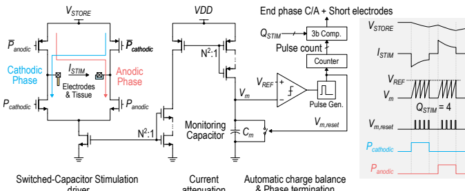
Fig. 6. Stimulation control stages for charge balancing and its operation. Current is copied with 16.6k reduction and threshold crossings are counted to track and balance charge.
