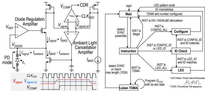
Fig. 3. TIA structure and its operation for optical reception with ambient light cancellation.
