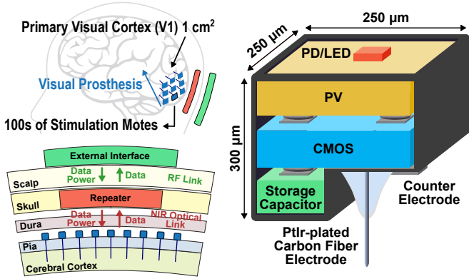
Fig. 1. Conceptual overview of the proposed free floating stimulation motes, their communication, and the 3D stack of chip layers with dimensions.
